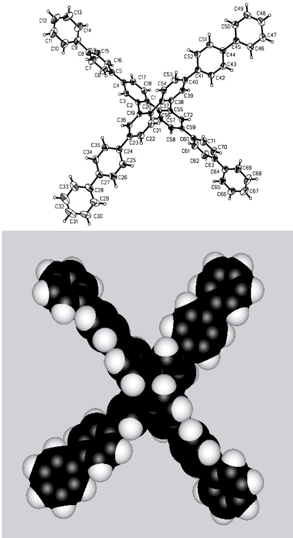
Figure 1. Molecular conformation for 4 as determined by a single crystal X-ray crystallography. The disordered molecules of solvent of crystallization (chloroform) are not shown. Top part: Ortep plot, carbon atoms are depicted with ellipsoids representing 50% probability level. Bottom part: space filling plot.
